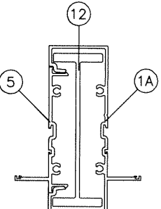
MULLION 'M2A'
