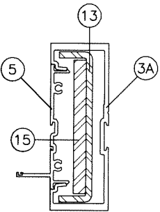
MULLION 'MD5'
