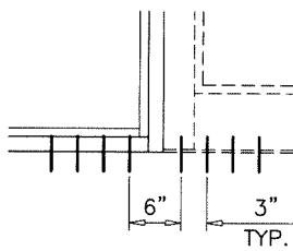
'C4' AT SILL ALL CASES
