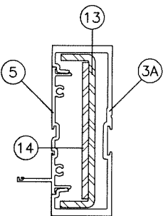
MULLION 'MD4'
