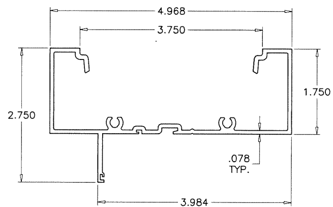
FRAME HEAD/SILL/JAMB/MULLION
