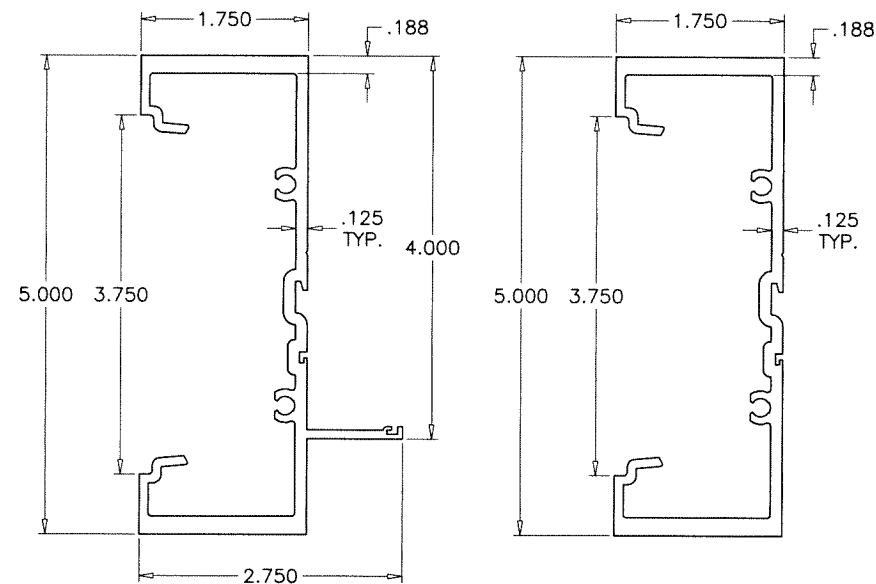
FRAME JAMB/MULLION
